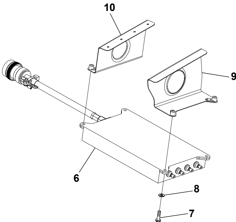
DETAIL B
