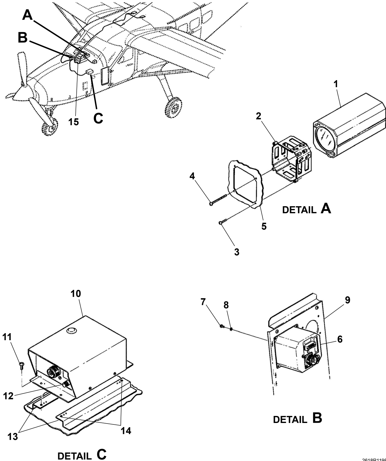
SPERRY 400 RMI INSTALLATION TYPE IN-404A Figure 01. (Sheet 1)
