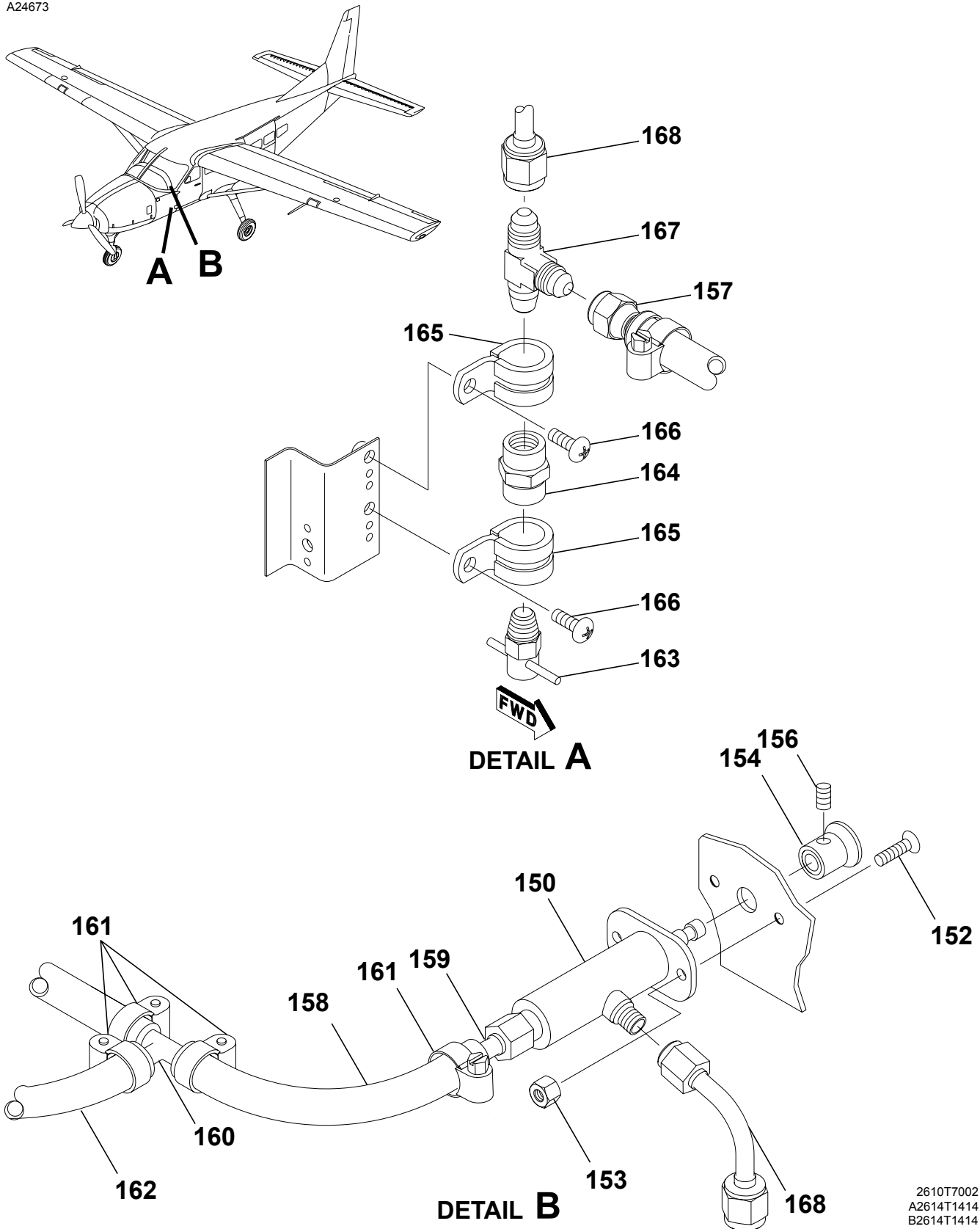
PITOT/STATIC SYSTEM Figure 01. (Sheet 3)
