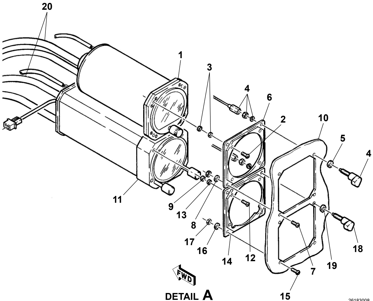
SPERRY 400B UNSLAVED GYRO INSTALLATION Figure 01. (Sheet 1)
