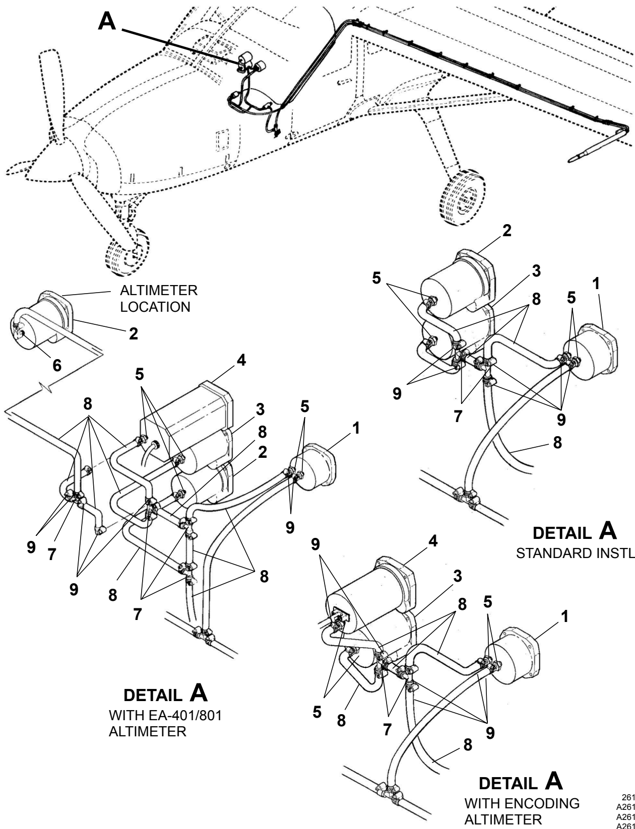
PITOT/STATIC SYSTEM Figure 01. (Sheet 1)
