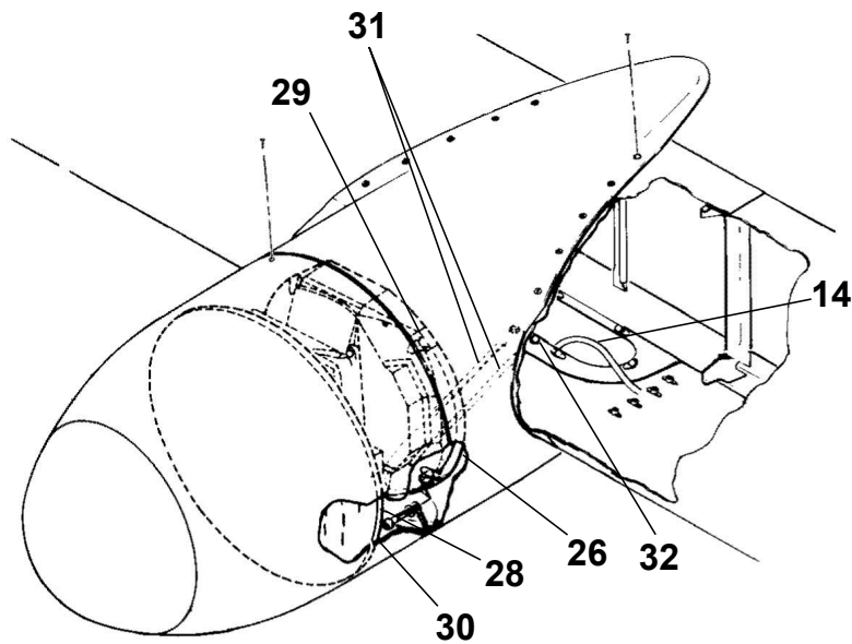
DETAIL C
