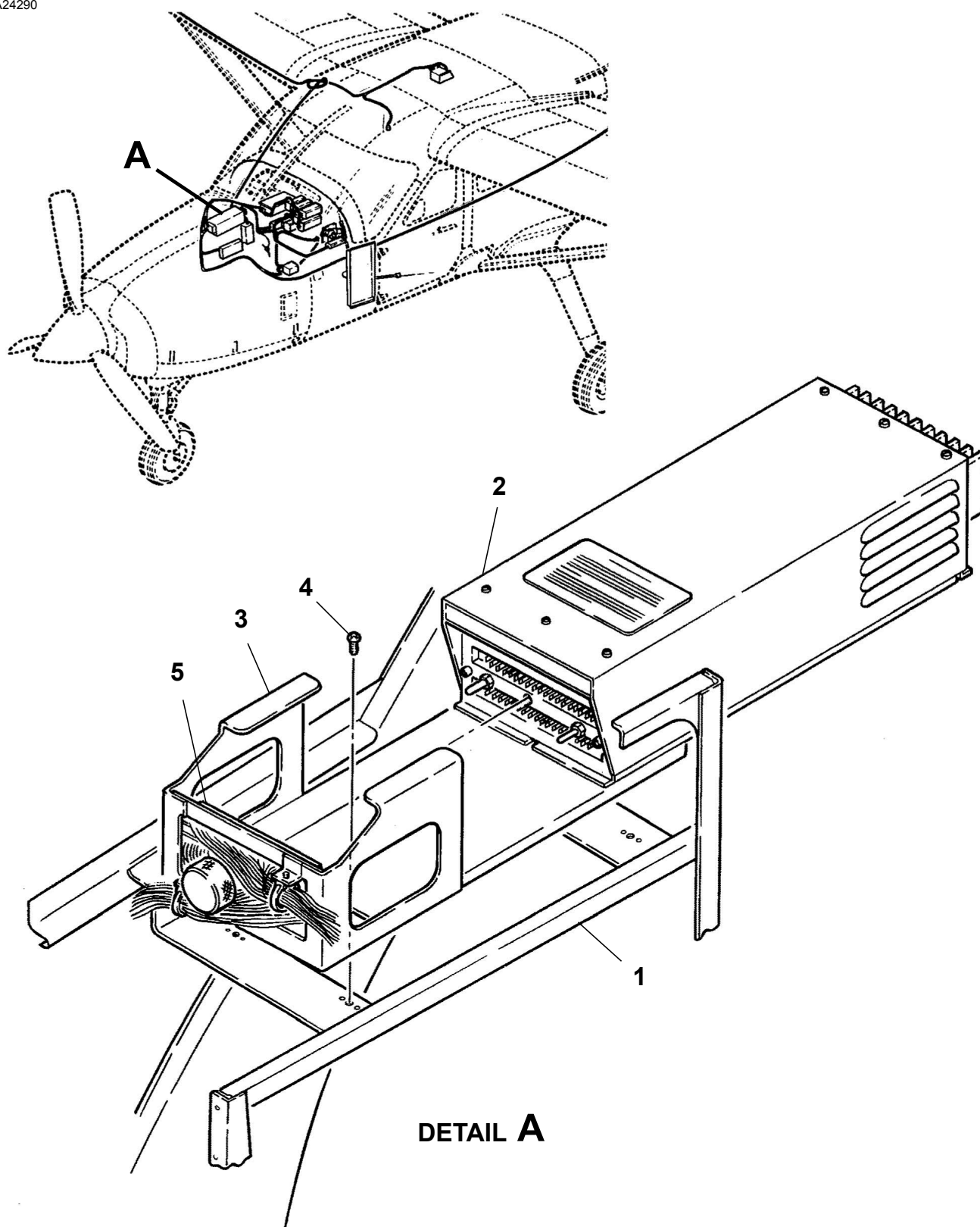
COMPUTER AMPLIFIER INSTALLATION Figure 01. (Sheet 1)
