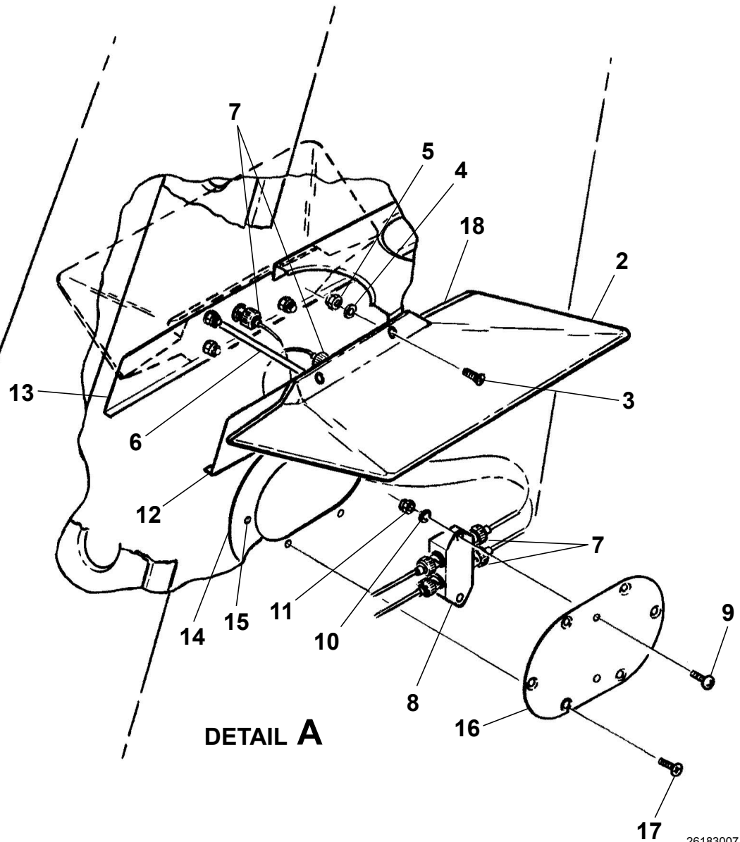
BALANCED LOOP ANTENNA INSTALLATION - NAV Figure 01. (Sheet 1)
