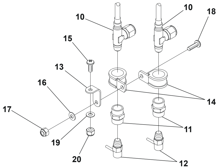
DETAIL B
