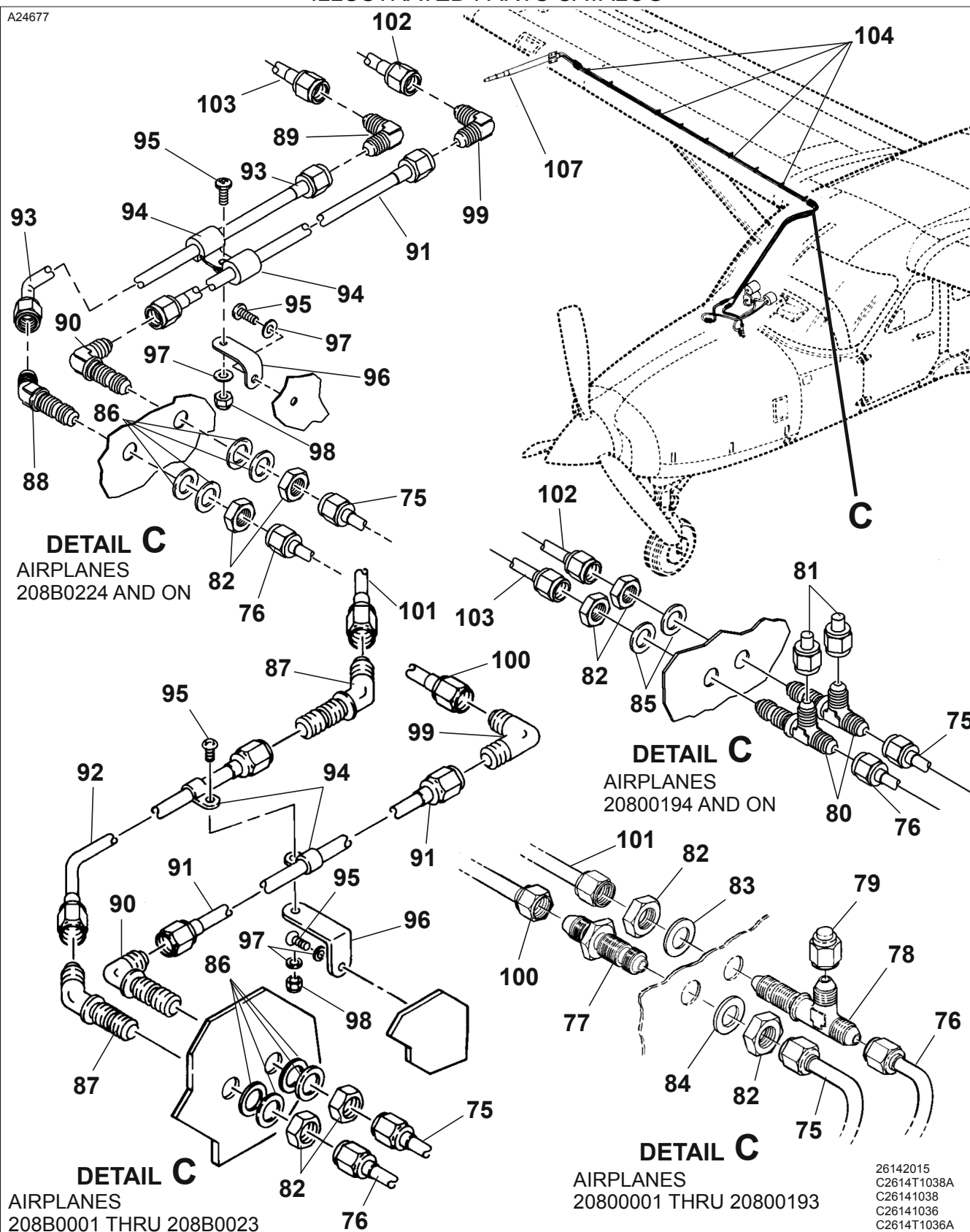
PITOT SYSTEM - RH FLIGHT PANEL Figure 01. (Sheet 2)
