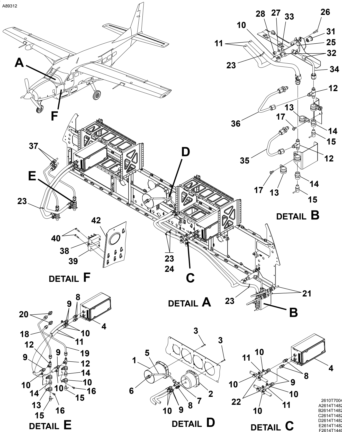
COCKPIT PITOT/STATIC SYSTEM Figure 02. (Sheet 1)
