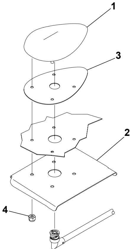
DETAIL B
