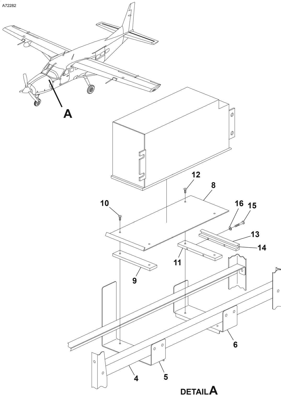
DME INSTALLATION Figure 03. (Sheet 1)
