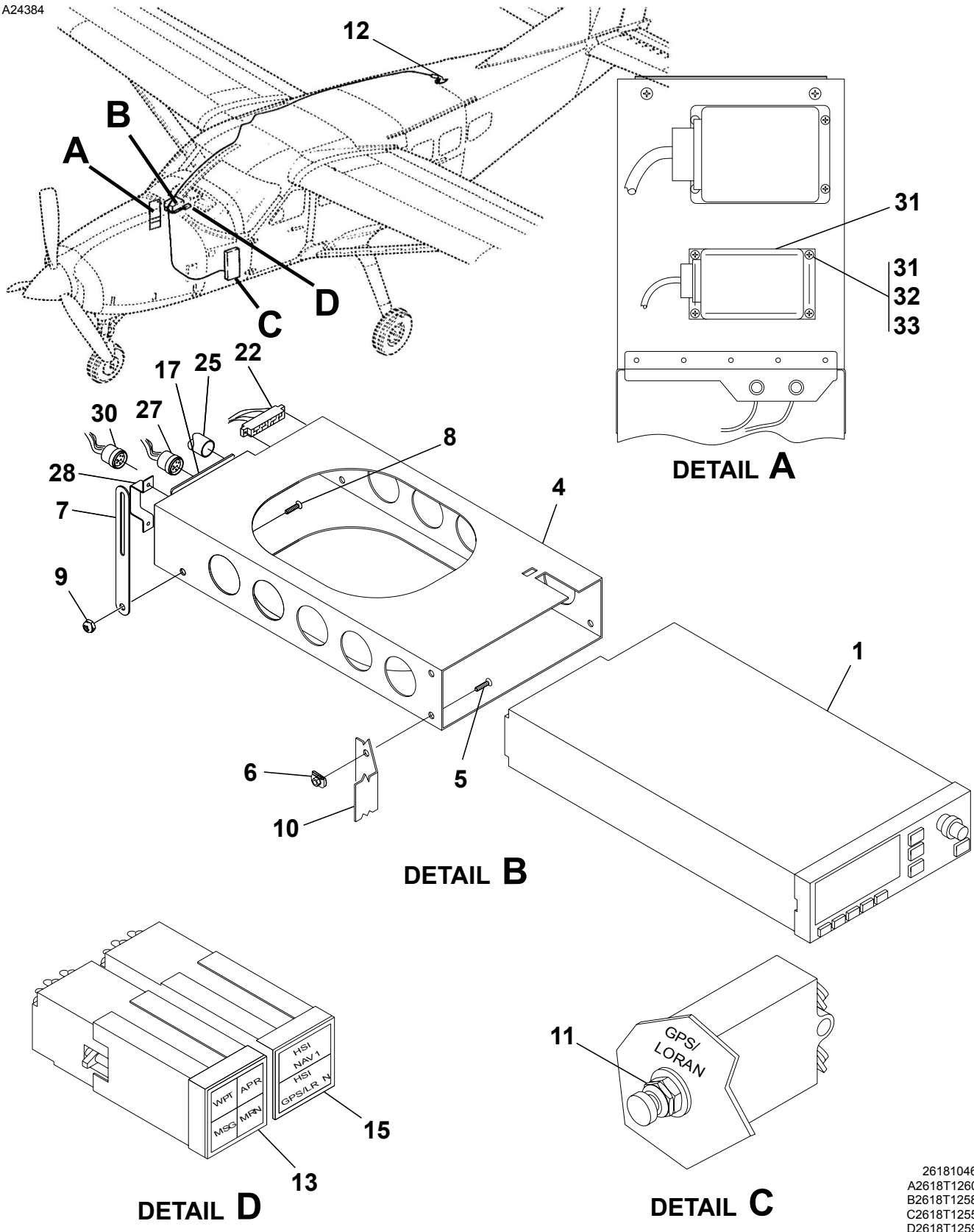
GPS TNL-2000T INSTALLATION Figure 01. (Sheet 1)
