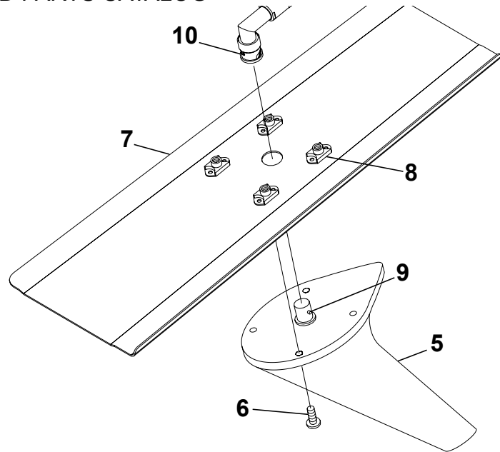
DETAIL B
