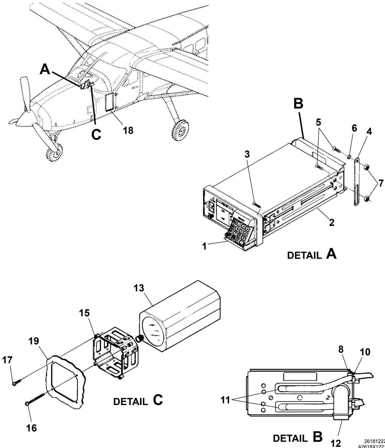
SPERRY AREA NAVIGATION RADIO INSTALLATION 400 - TYPE RN-479A Figure 01. (Sheet 1)
