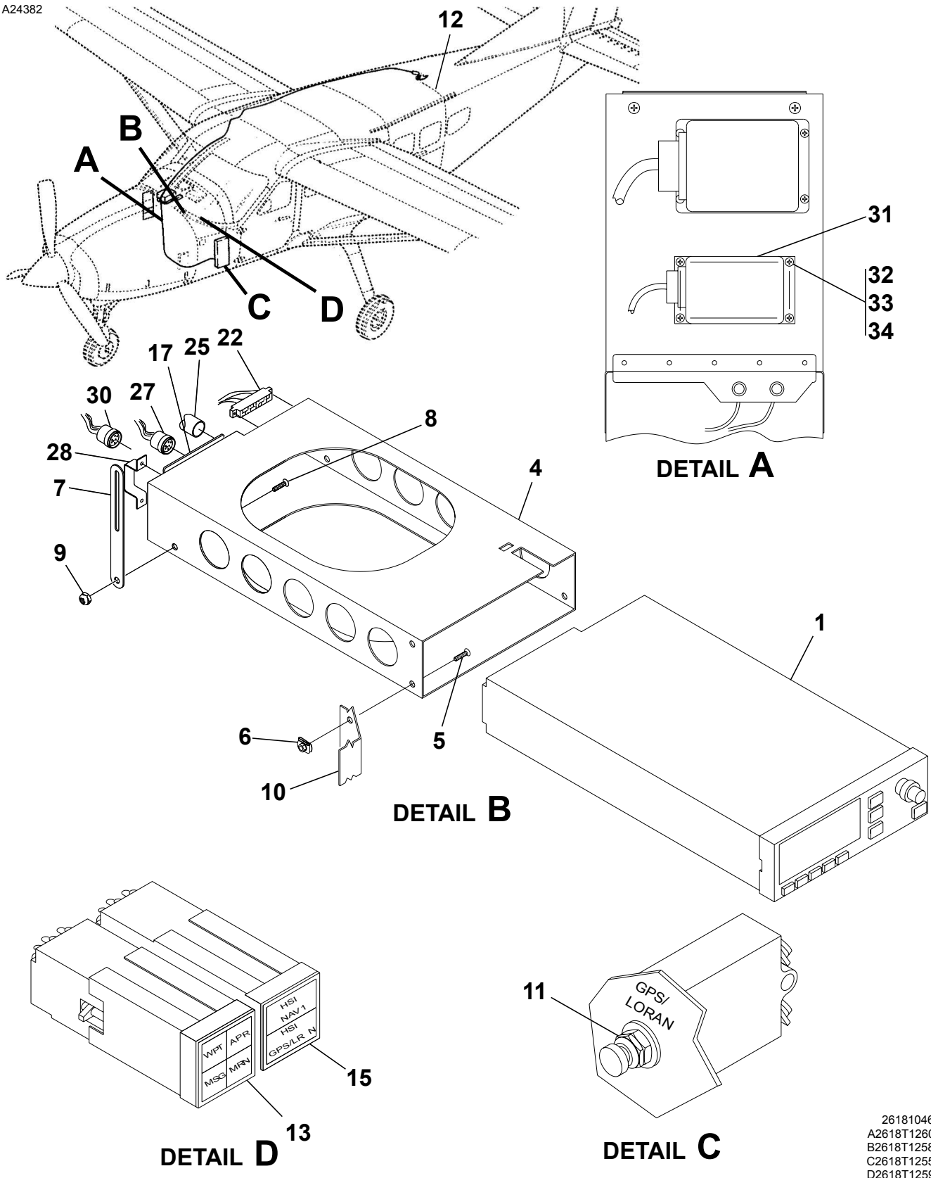
GPS/LORAN TNL-3000T INSTALLATION Figure 01. (Sheet 1)
