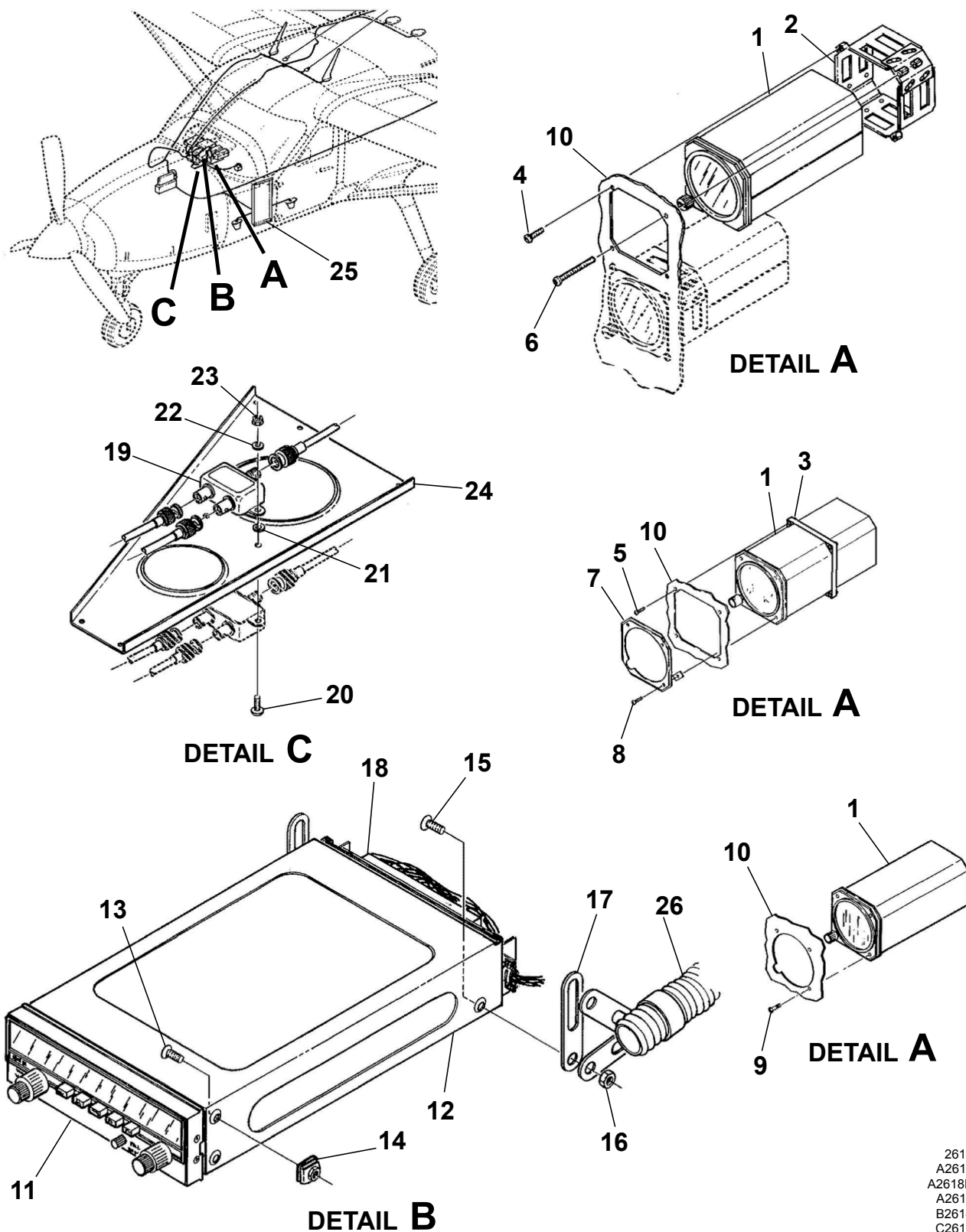
KING RNAV RADIO INSTALLATION - KNS81 Figure 01. (Sheet 1)
