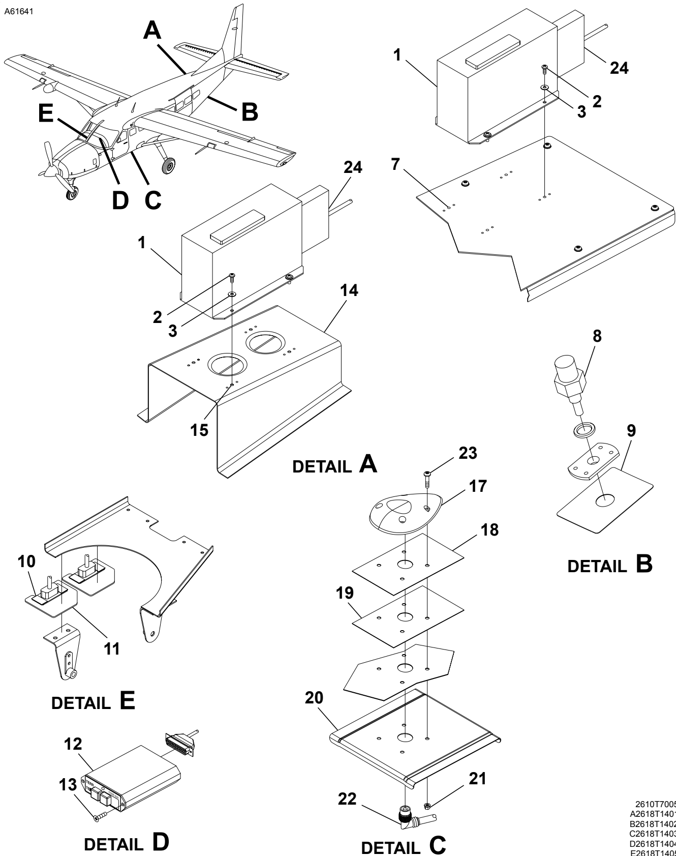
EGPWS INSTALLATION Figure 01. (Sheet 1)
