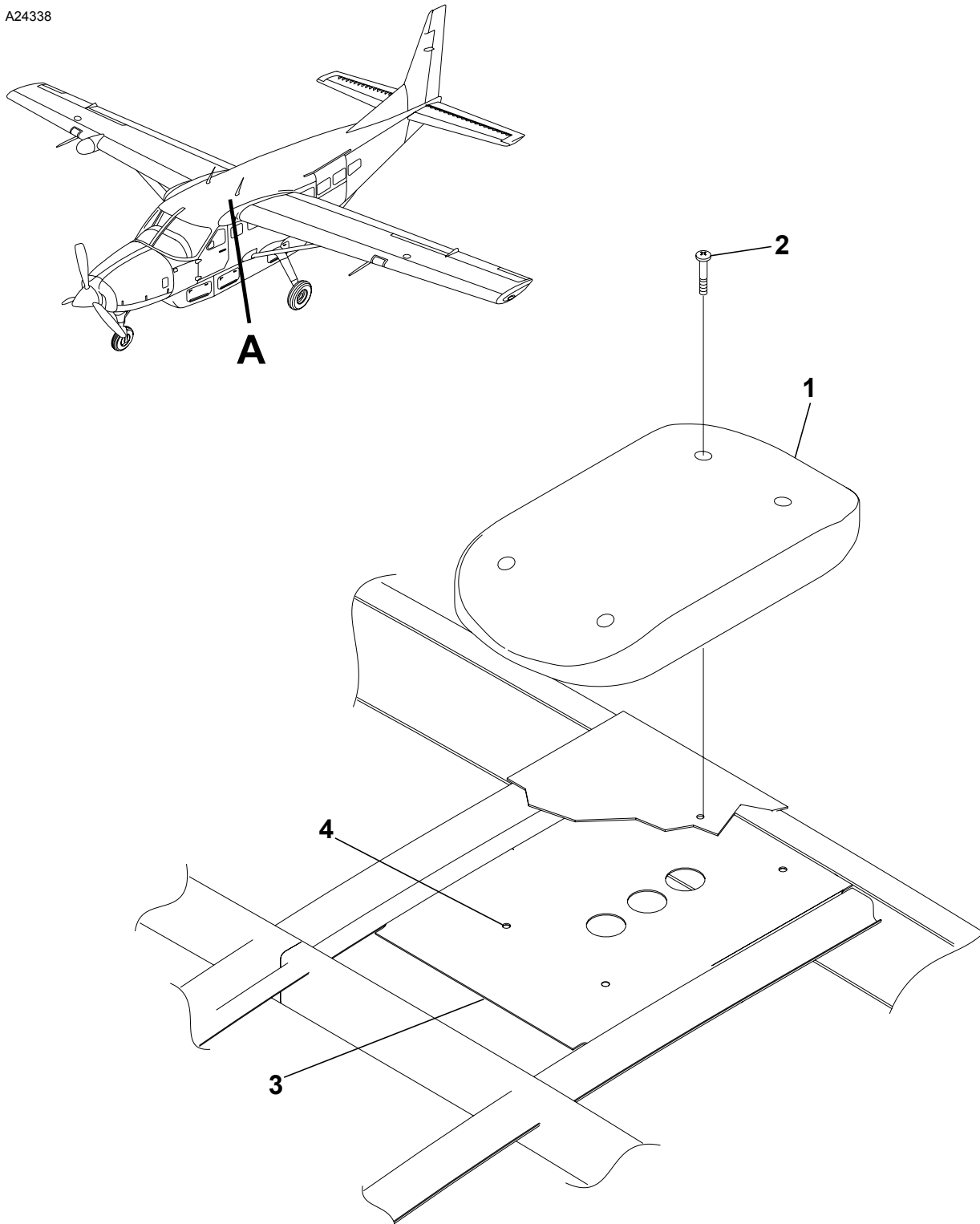
DETAIL A
