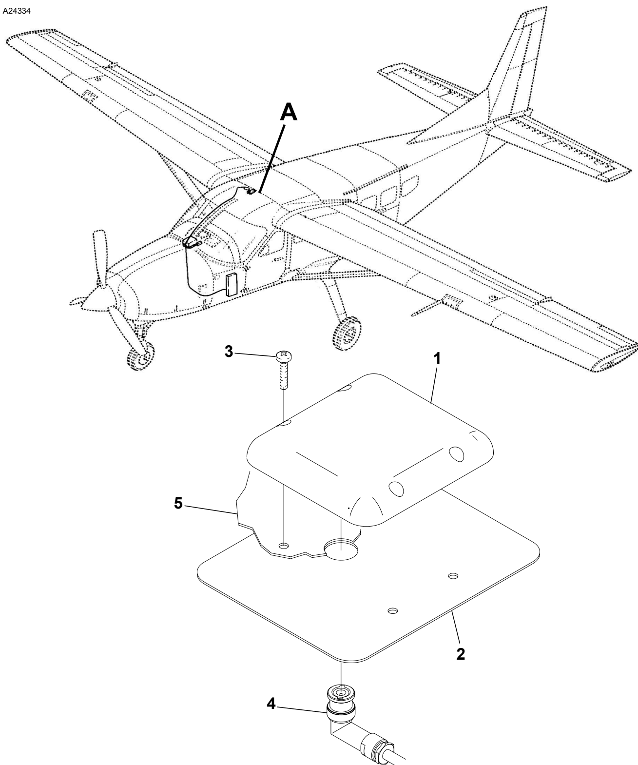
DETAIL A
