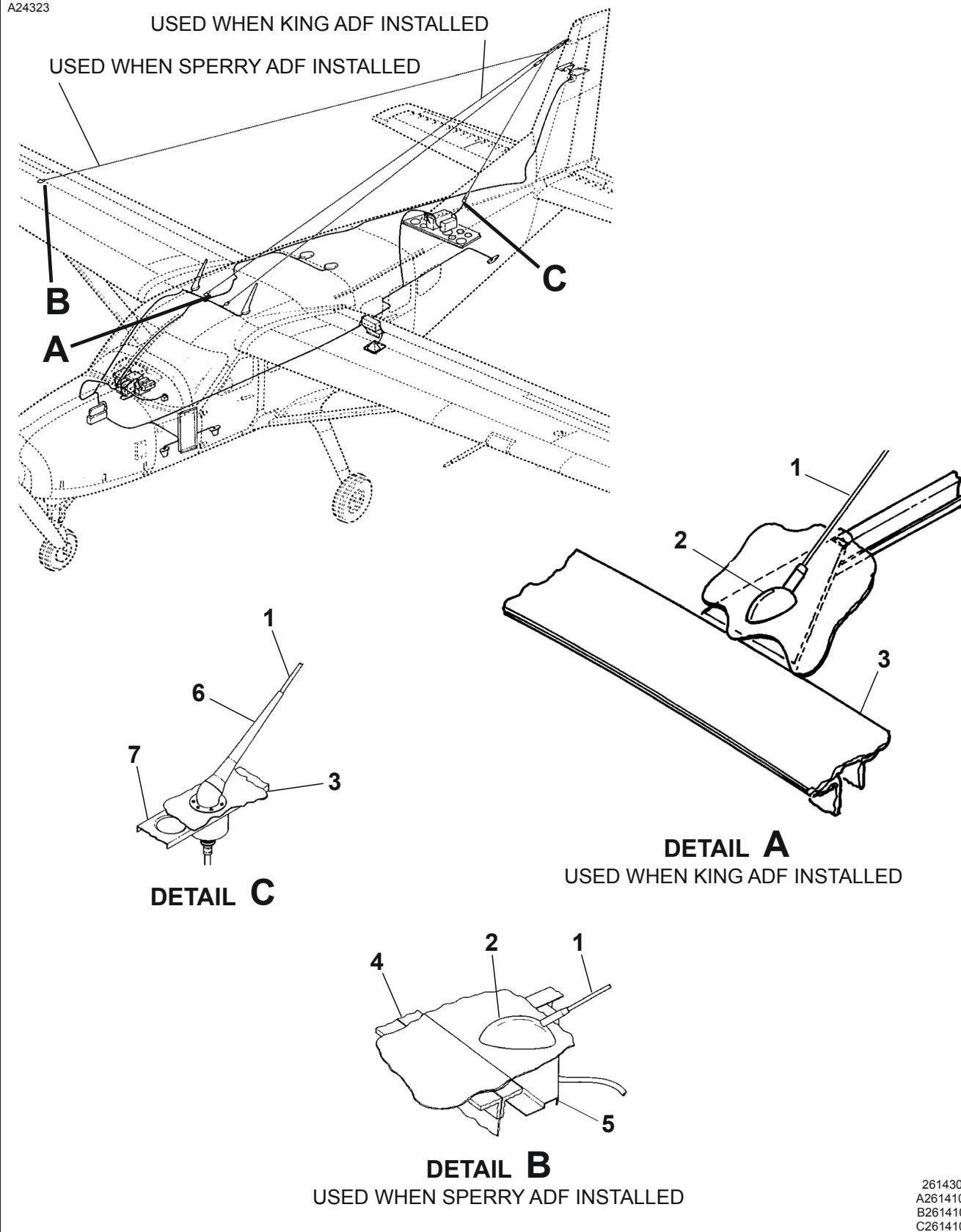
KING HF RADIO ANTENNA INSTALLATION - TYPE KHF 950 Figure 04. (Sheet 1)
