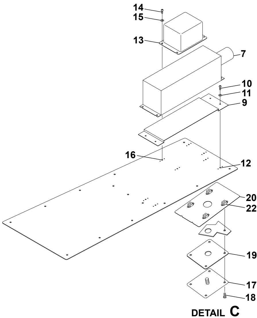
RADAR ALTIMETER INSTALLATION Figure 08A. (Sheet 1)
