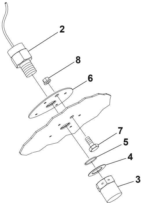
DETAIL B
