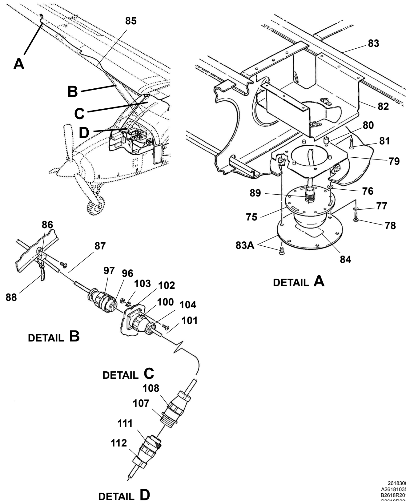
FLUX DETECTOR INSTALLATION Figure 01. (Sheet 2)
