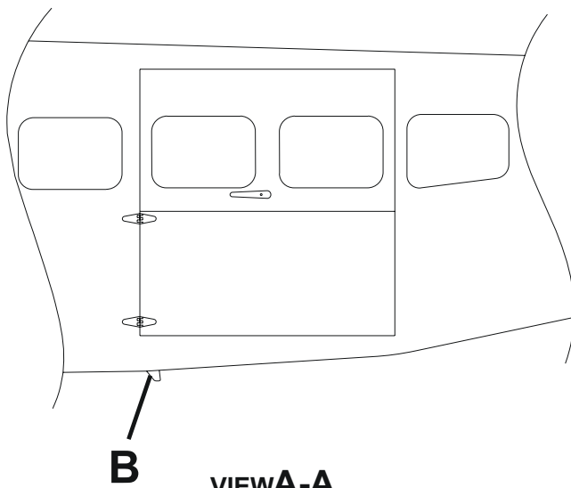
DME ANTENNA INSTALLATION Figure 02. (Sheet 1)
