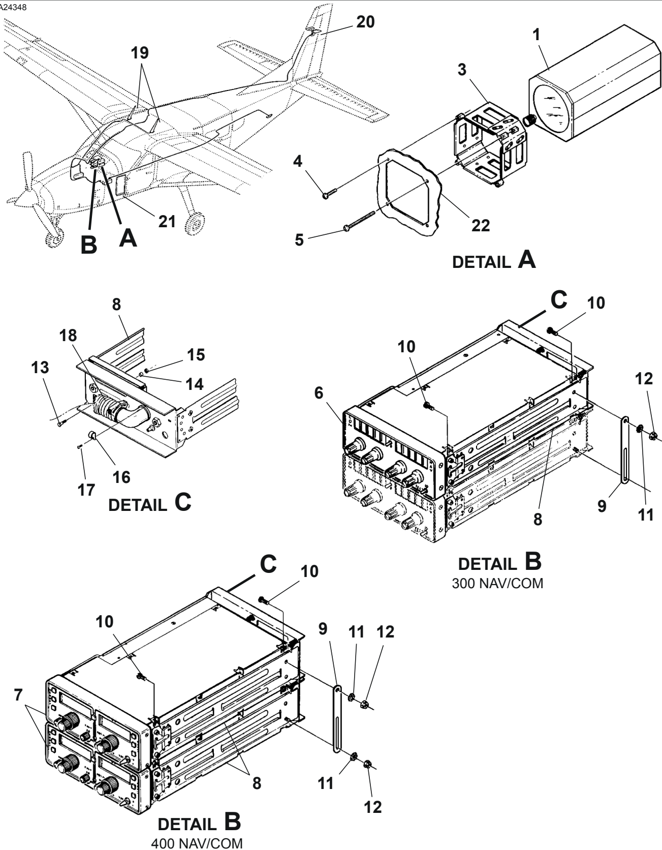
SPERRY NAV/COM RADIO INSTALLATIONS Figure 05. (Sheet 1)
