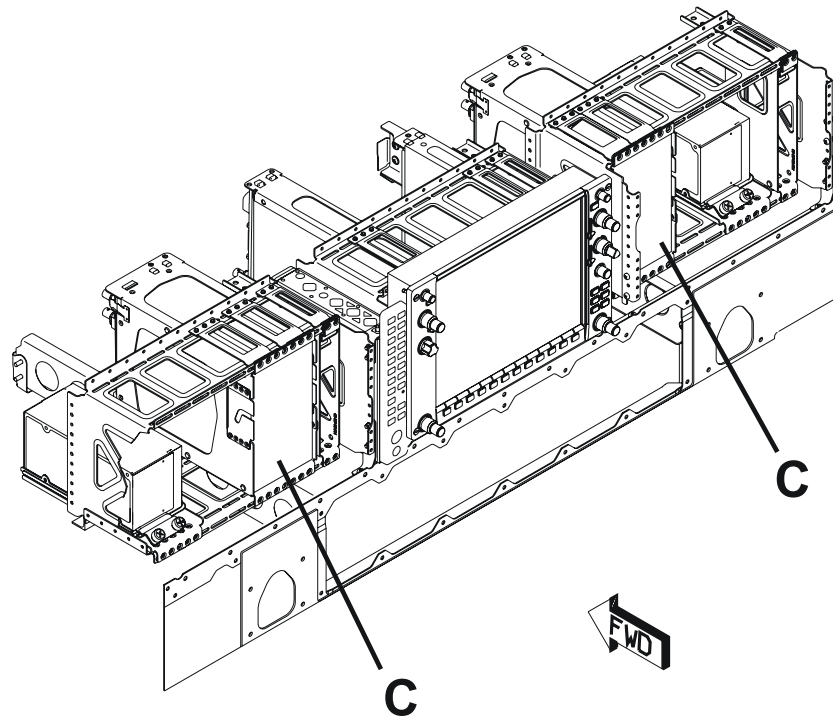
DETAIL B
