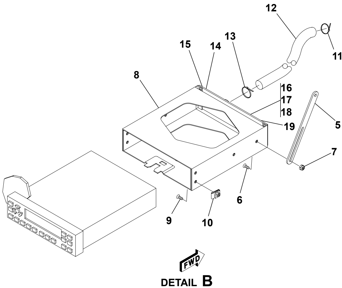
GARMIN GTX-327 INSTALLATION Figure 01. (Sheet 1)
