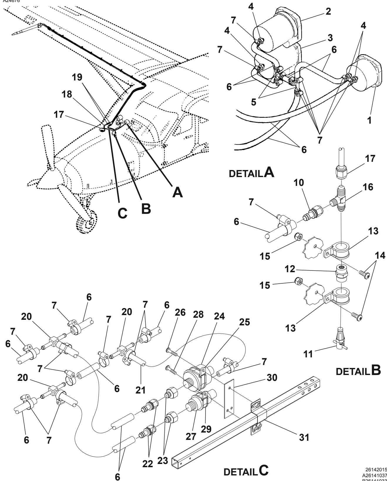
PITOT SYSTEM - RH FLIGHT PANEL Figure 01. (Sheet 1)
