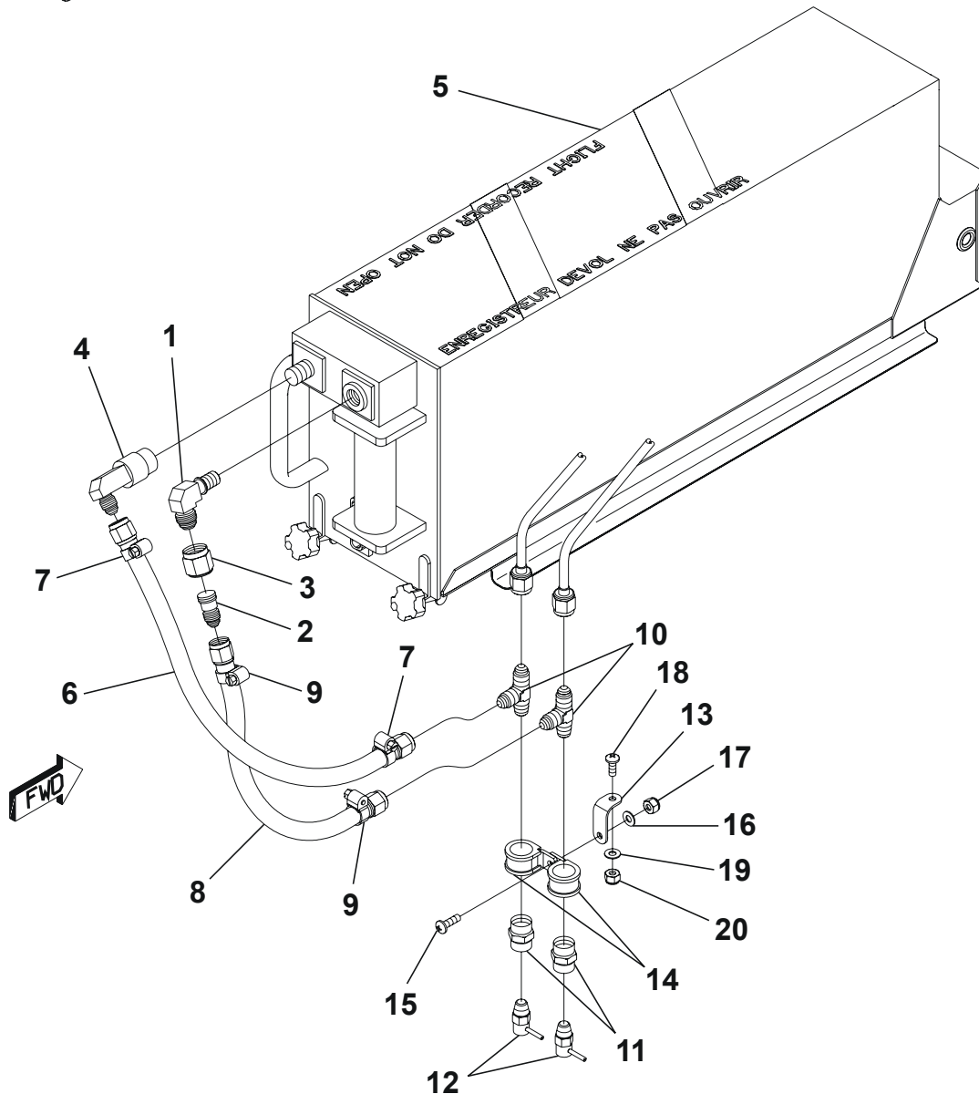
PITOT/STATIC INSTALLATION WITH FLIGHT DATA RECORDER Figure 03. (Sheet 1)
