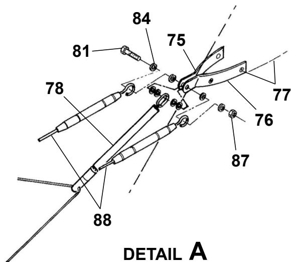
KING HF RADIO ANTENNA INSTALLATION - TYPE KHF 950 Figure 04. (Sheet 2)
