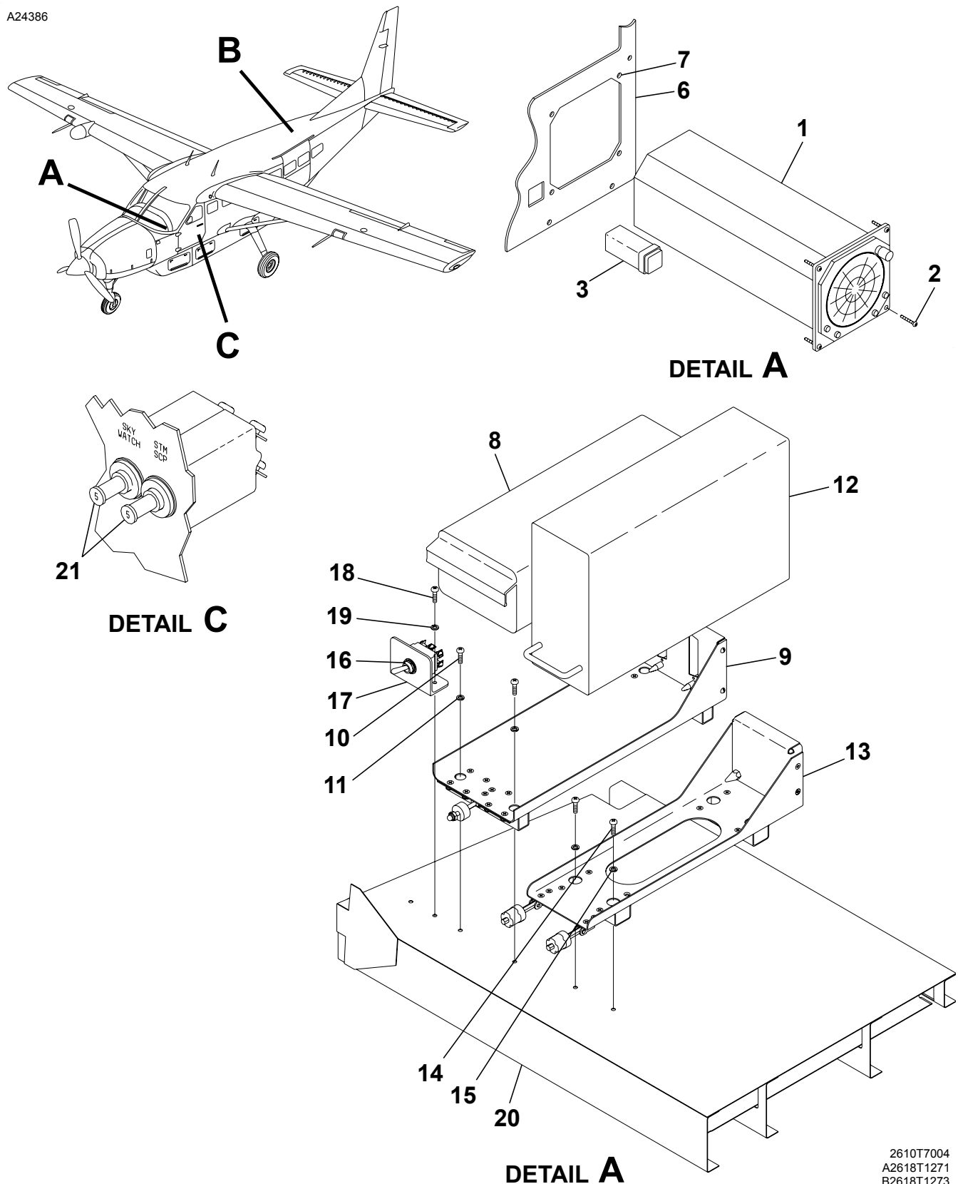
STORMSCOPE AND SKYWATCH INSTALLATION Figure 02. (Sheet 1)
