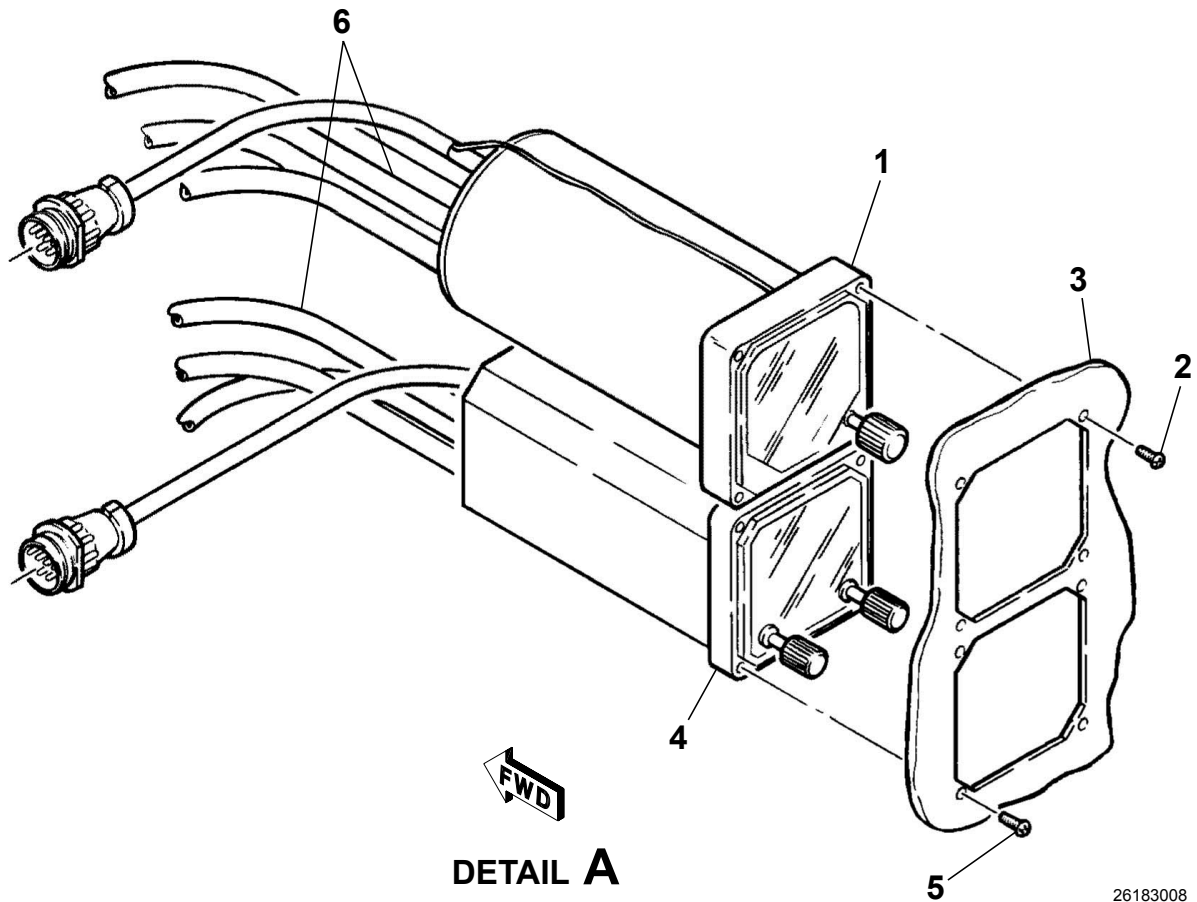
SPERRY 400B SLAVED GYRO INSTALLATION Figure 01. (Sheet 1)
