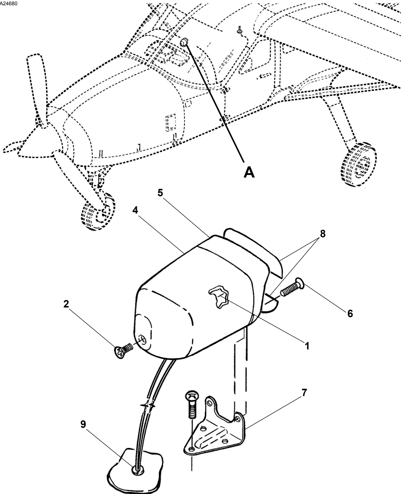
COMPASS INSTALLATION Figure 01. (Sheet 1)
