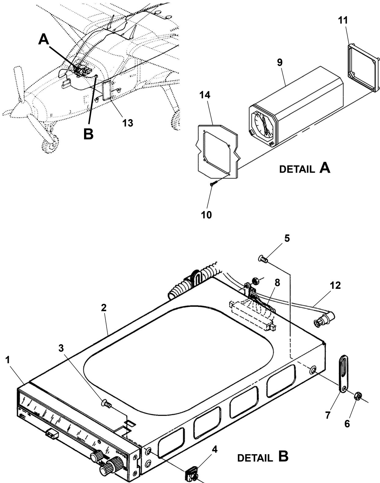
KING ADF RADIO INSTALLATION WITH RMI Figure 02. (Sheet 1)
