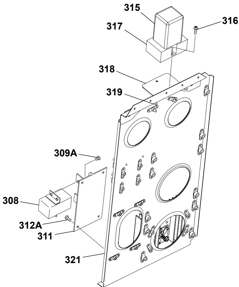
DETAIL B
