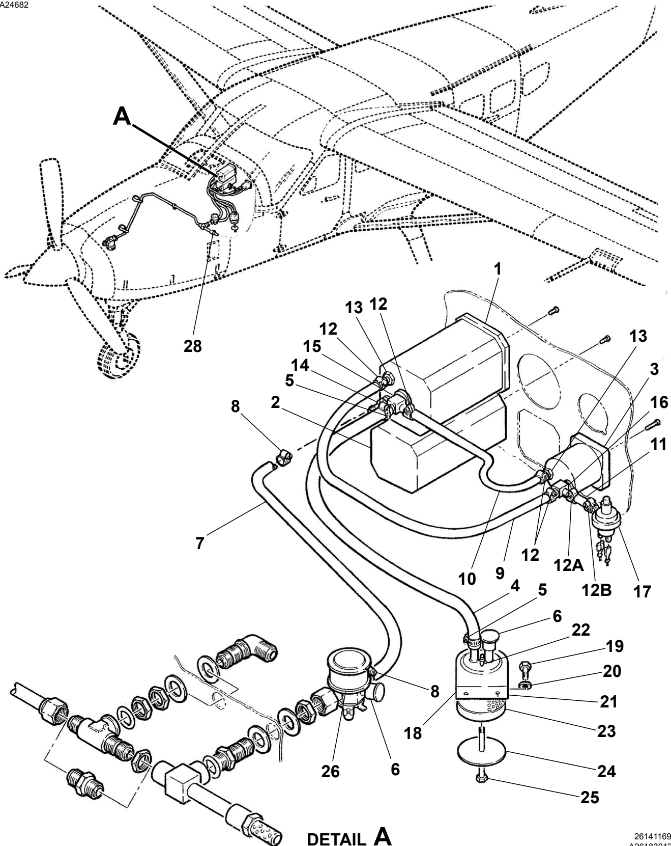
GYROS INSTALLATION Figure 02. (Sheet 1)
