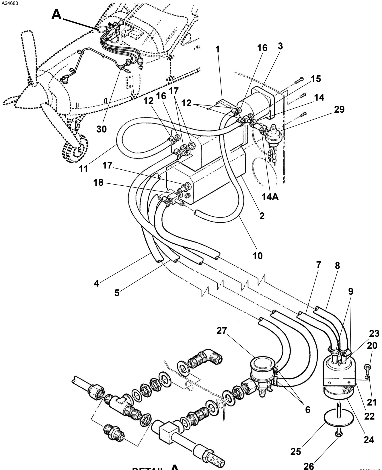
GYROS INSTALLATION - RIGHT FLIGHT PANEL Figure 01. (Sheet 1)
