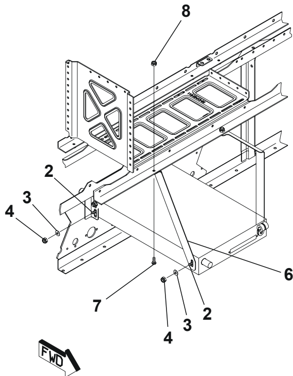
DETAIL B
