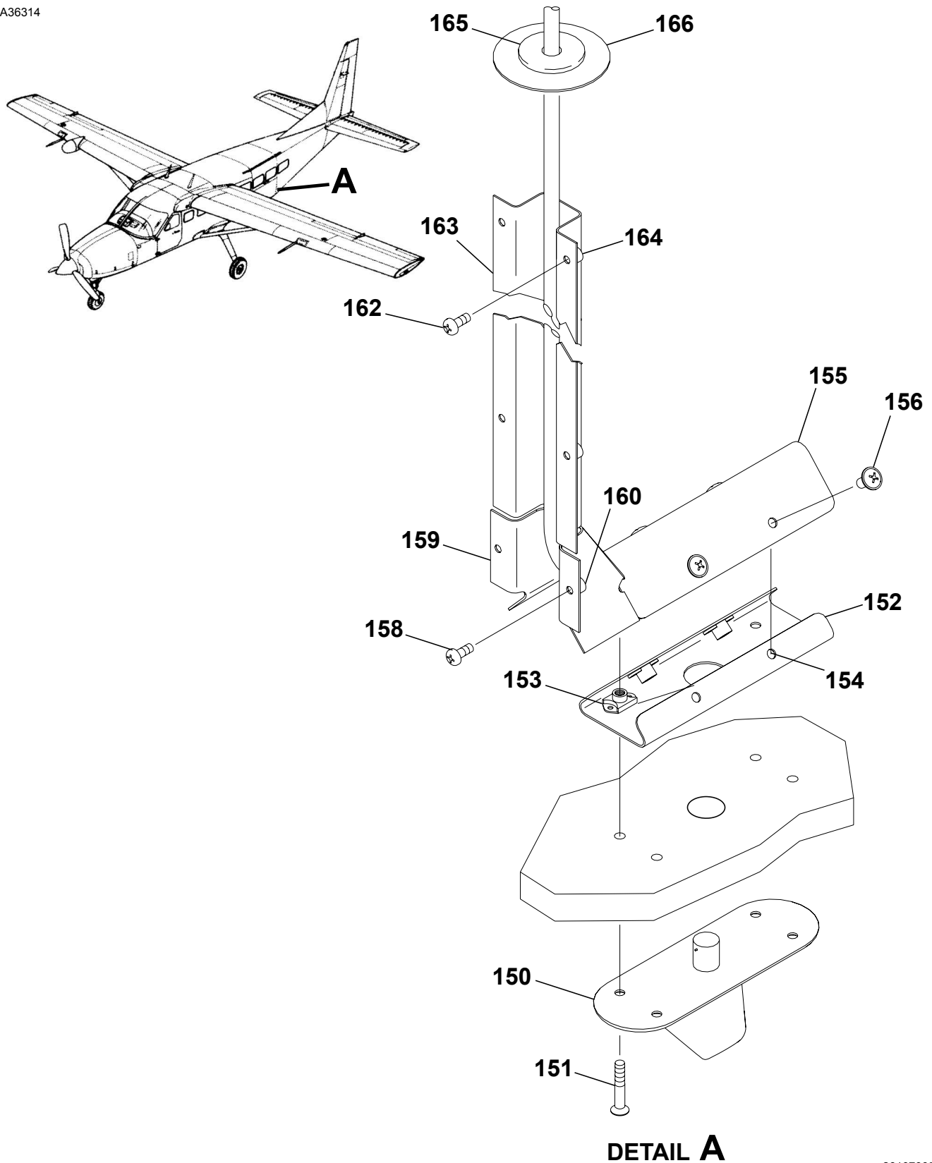
GARMIN GTX-327 INSTALLATION Figure 01. (Sheet 3)
