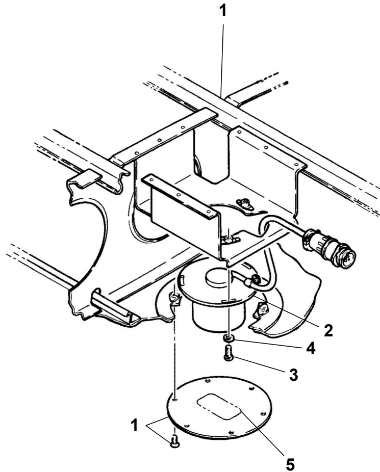
DETAIL A
