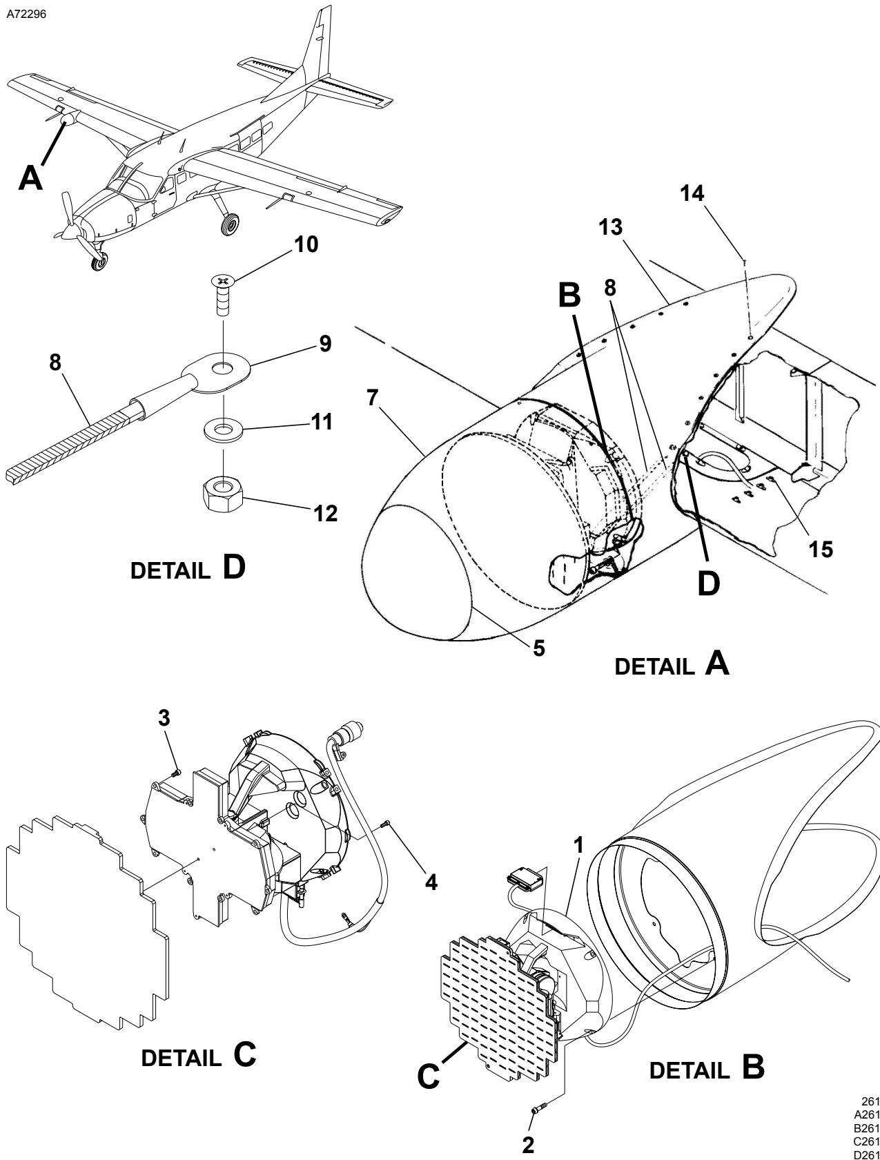
GWX 68/70/75 WEATHER RADAR INSTALLATION Figure 01. (Sheet 1)
