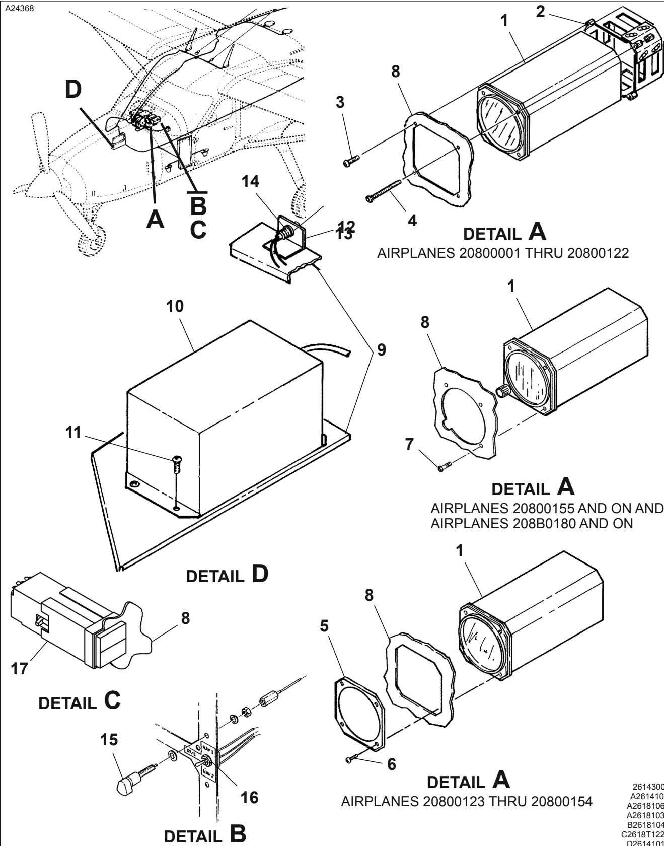
KING RMI INSTALLATION - TYPE KI229 Figure 01. (Sheet 1)
