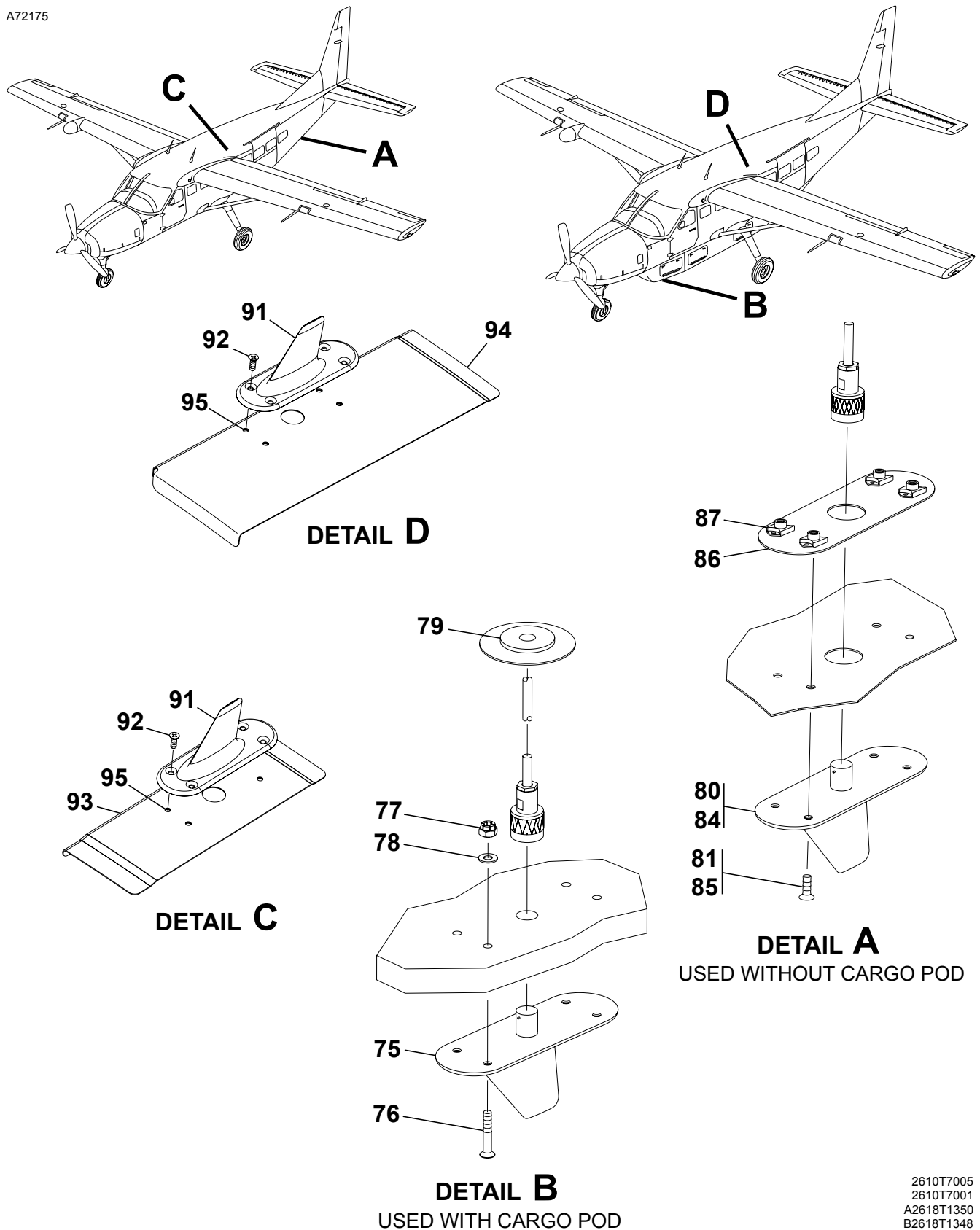
GARMIN GTX-33 TRANSPONDER INSTALLATION WITH OR WITHOUT POD Figure 01. (Sheet 2)
