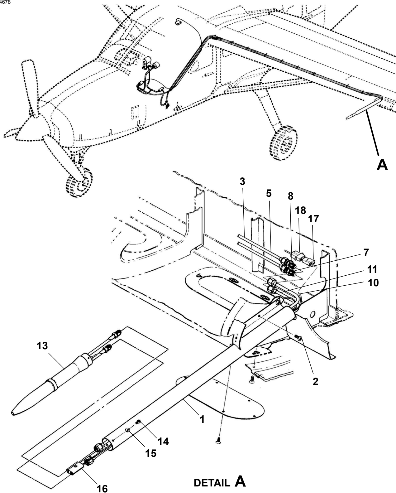
PITOT TUBE INSTALLATION Figure 01. (Sheet 1)
