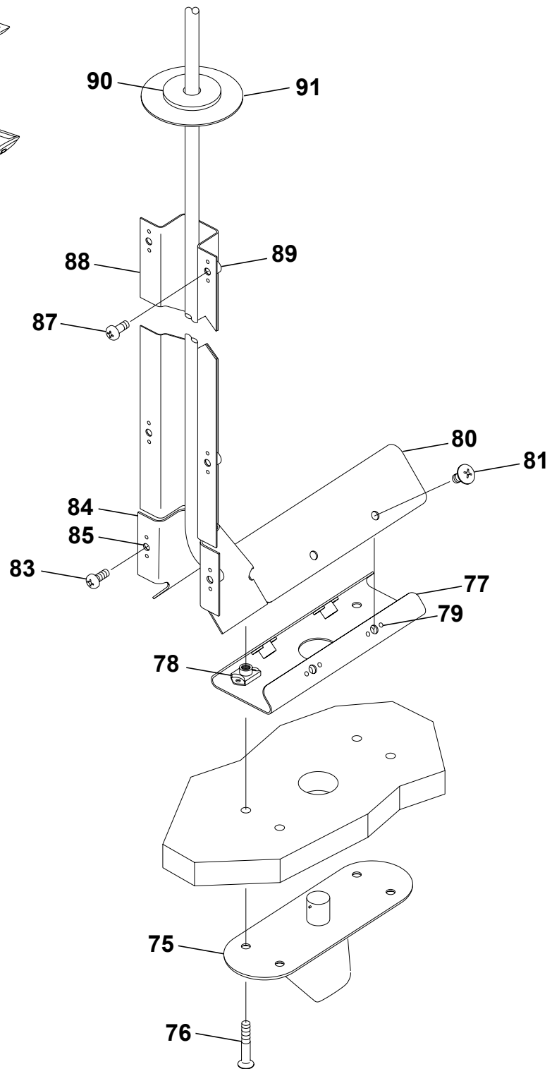
DME ANTENNA INSTALLATION Figure 02. (Sheet 2)
