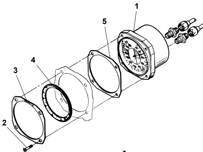
DETAIL A TRUE AIRSPEED INSTALLATION
