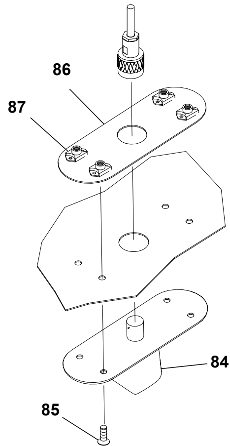
DETAIL A
