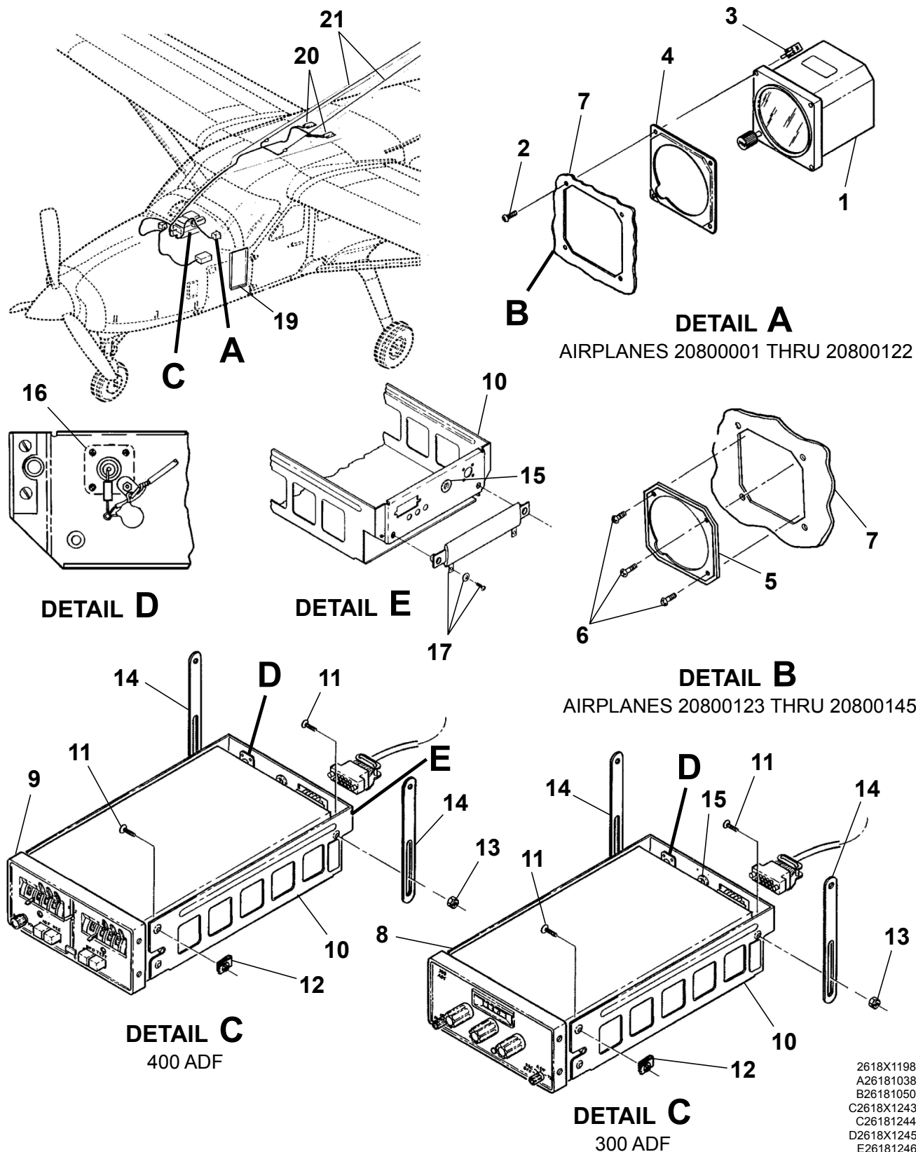
SPERRY ADF RADIO INSTALLATION Figure 01. (Sheet 1)
