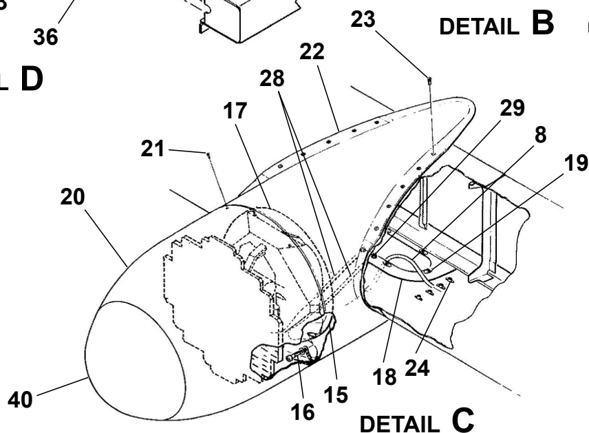
NARCO WEATHER RADAR INSTALLATION - TYPE KWX56 Figure 01. (Sheet 1)
