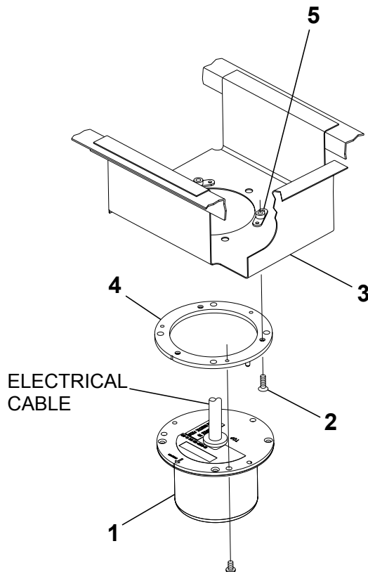
DETAIL A
