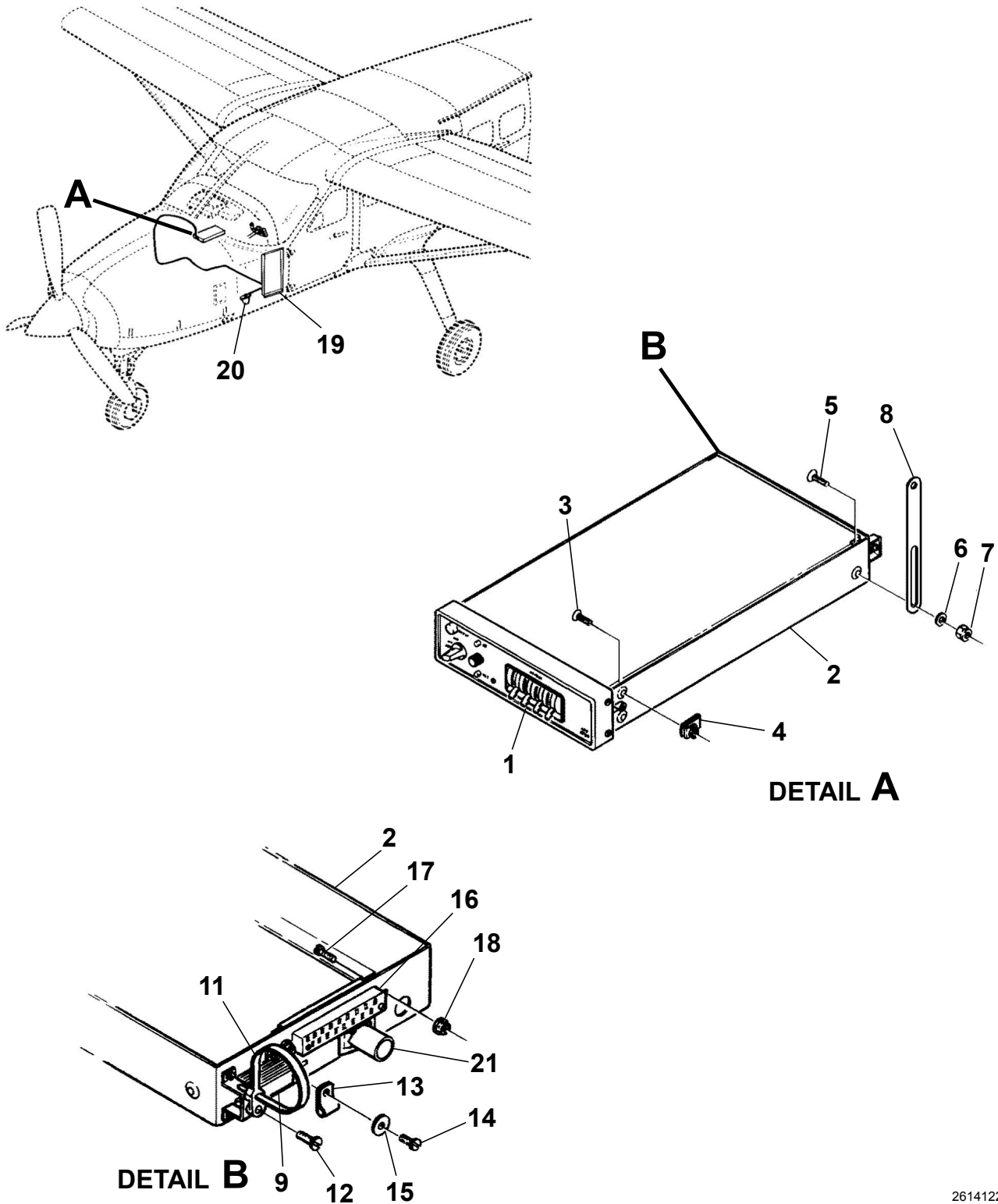
SPERRY TRANSPONDER INSTALLATION 400 - TYPE RT-459A Figure 01. (Sheet 1)
