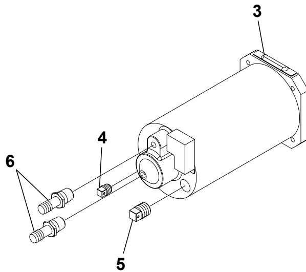
DETAIL B
