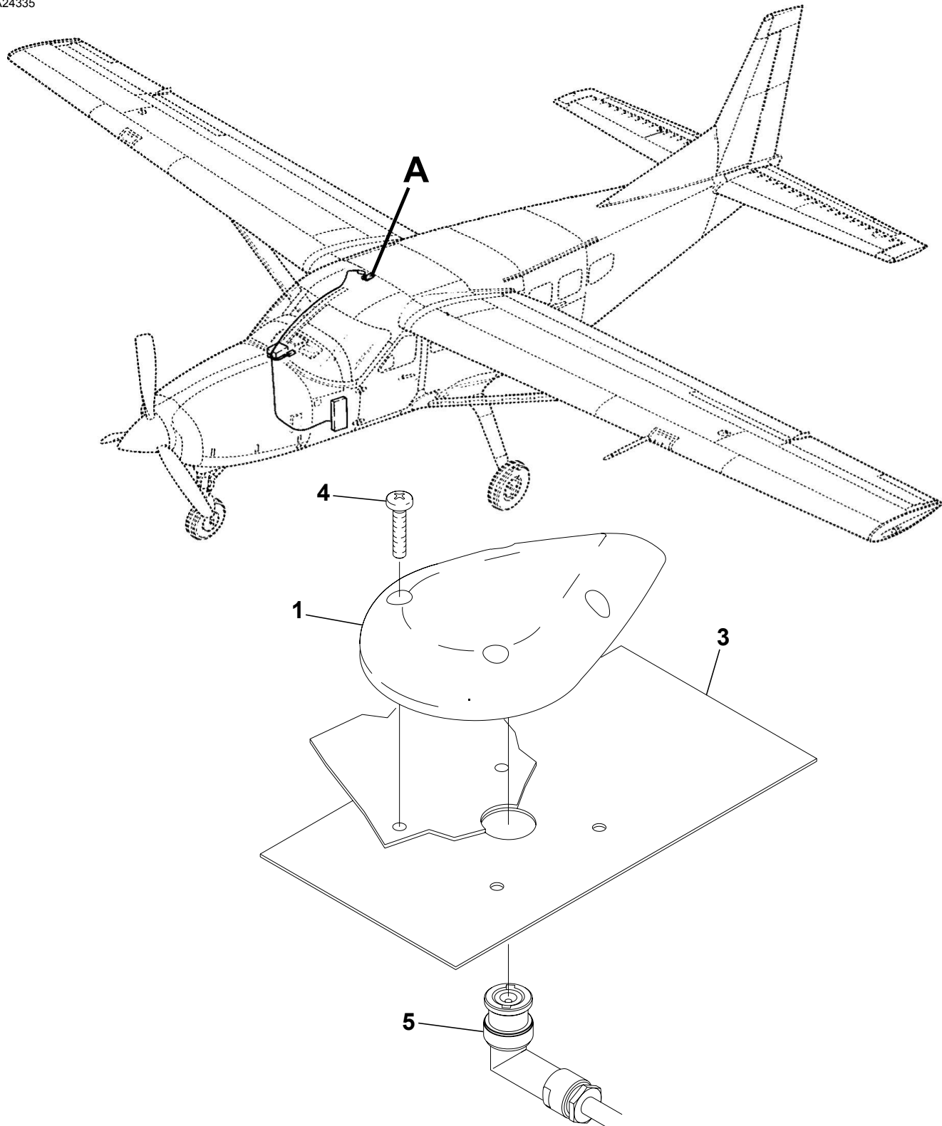
GPS ANTENNA INSTALLATION Figure 01. (Sheet 1)
