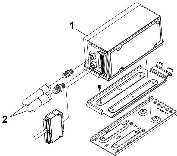
DETAIL C
