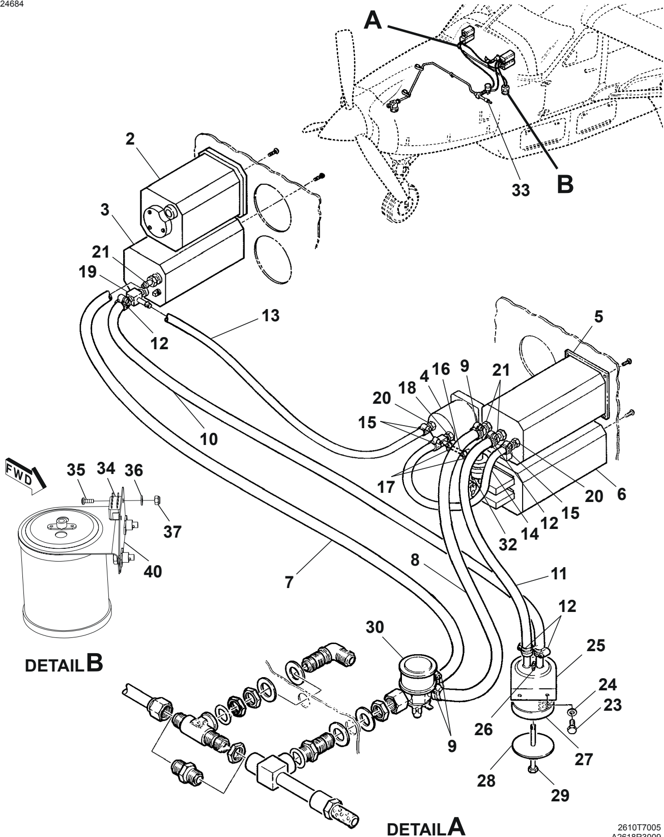
GYRO INSTALLATION - VACUUM Figure 02. (Sheet 1)
