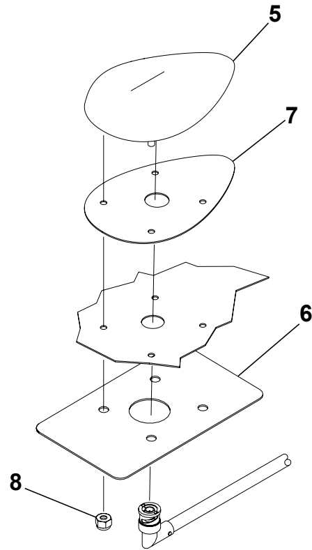
DETAIL A
