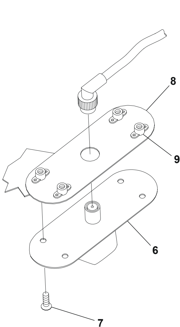
DETAIL B
