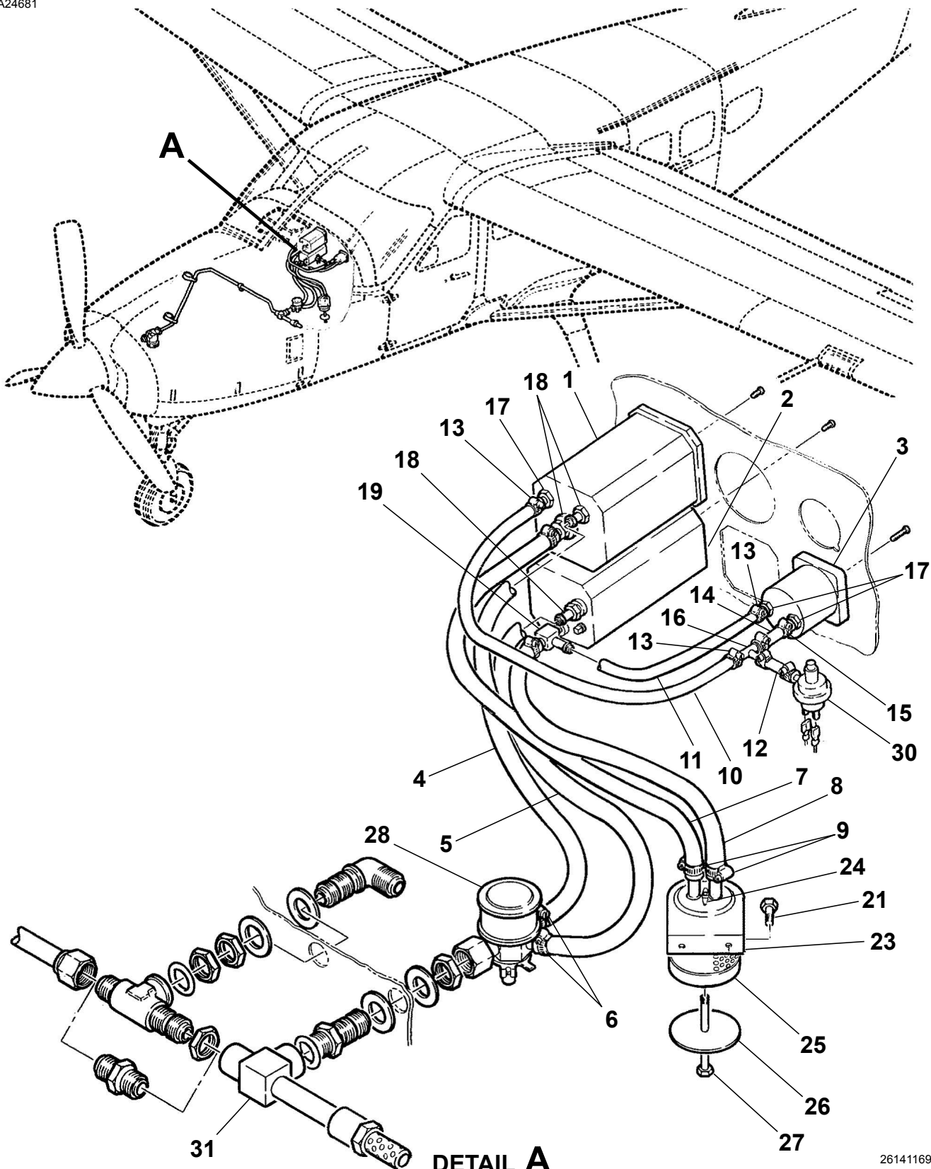
GYROS INSTALLATION Figure 01. (Sheet 1)
