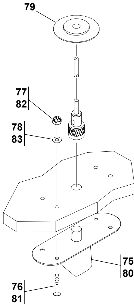
DETAIL B
