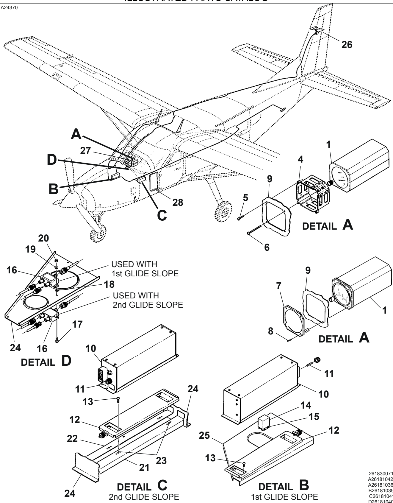
SPERRY 400 GLIDESLOPE INSTALLATION - TYPE R-443B Figure 01. (Sheet 1)
