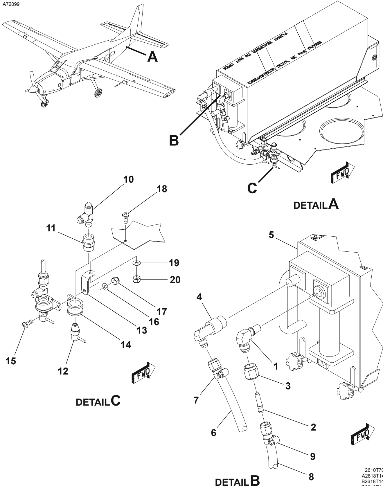
PITOT/STATIC INSTALLATION WITH FLIGHT DATA RECORDER Figure 02. (Sheet 1)
