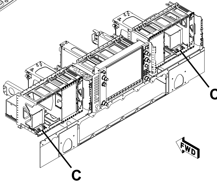
DETAIL B
